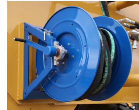
Hose Reel: COXREELS: One-piece, all CNC robotically welded steel "A" frame construction; custom design for Premier Tanks
