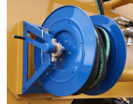
One piece, all CNC robotically welded steel "A" frame construction
